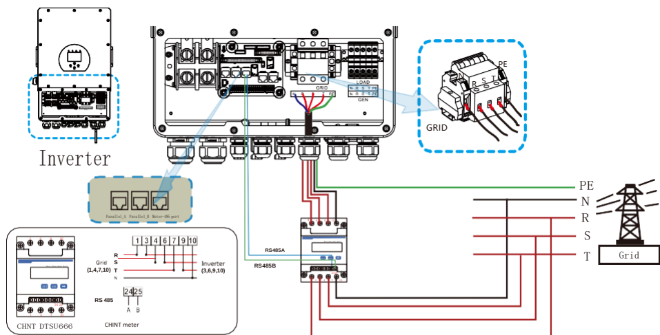
Definition of RJ45 Port Pin for Meter-485
