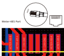
Definition of RS45 Port Pin for Meter-485
